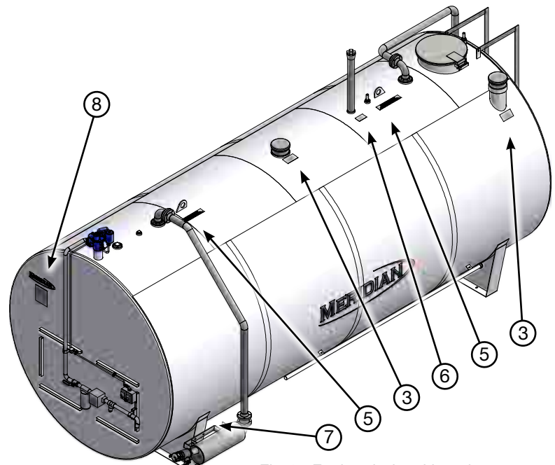
Fig 4 - Fuel tank decal location
