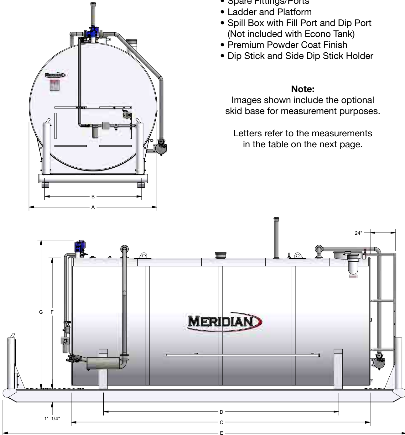
Fig 2 - Tank measurements, shown with optional skid
